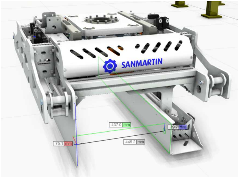
Tool without product total opening 437mm
