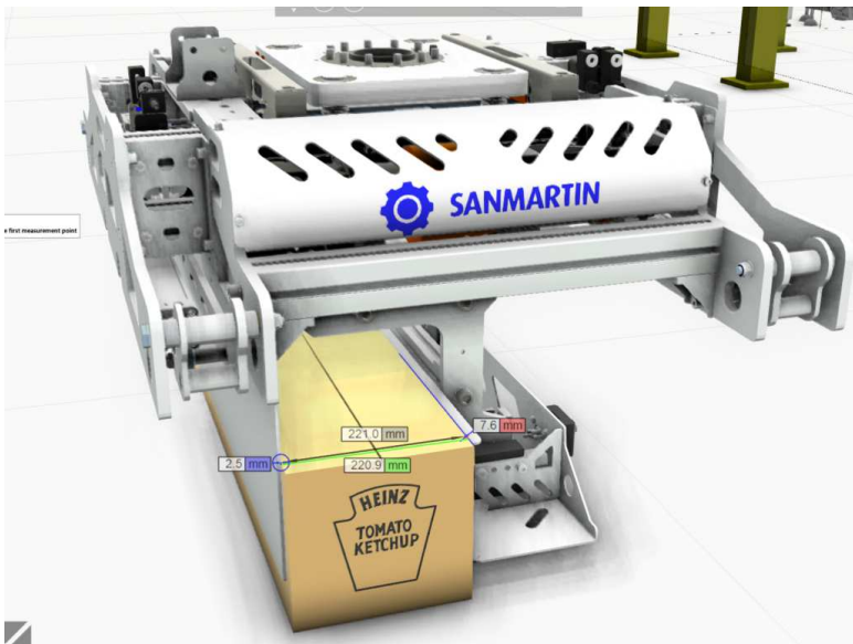
Tool with longitudinal boxes 221 mm opening
